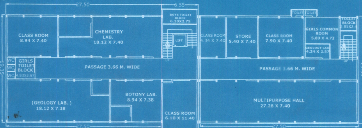
EXISTING FIRST FLOOR PLAN BLOCK-A
